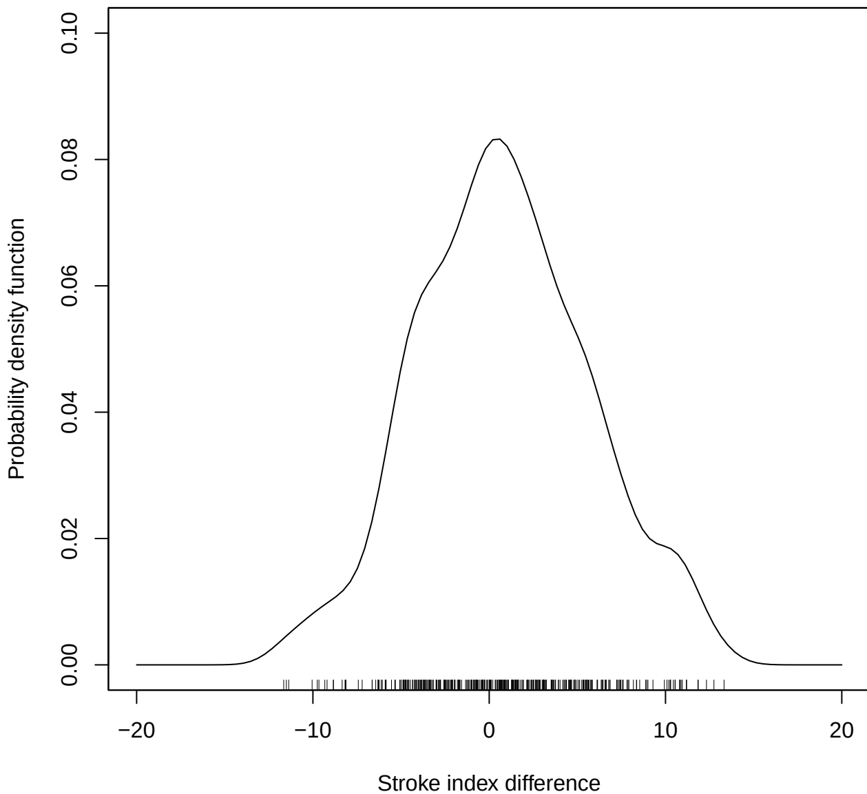
Kernel density estimation ('CV' h = 1.141399)
